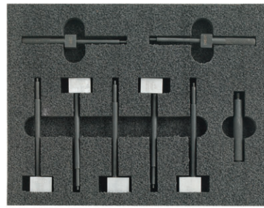
Detroit Diesel Injector Height Gauge Set Used to set Injector Body Height to the injector follower for proper fuel injector timing. For Detroit Diesel two Cycle 71, two cycle 92, series 60 and DDEC IV Engines. OTC- 5870
